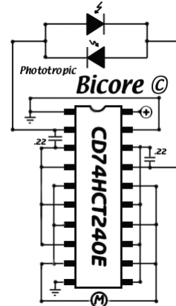
Schematic courtesy BEAM-Online
